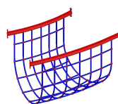
PD-6.C - Curved Tibetan bridge NR 1 The net is made of steel strands rope, 18 mm diameter, covered with a colored nylon braid, highly resistant. The knots are covered with shell-shape protections
