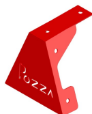
CTSA0010 - Swing Bracket NR 2 Bracket: Bracket to attach the legs and main girder made by steel
